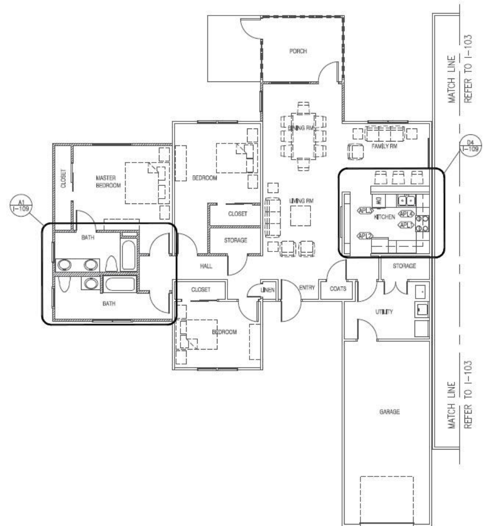
UNIT B - FF&E PLAN SCALE: 3/16" = 1'-0"
